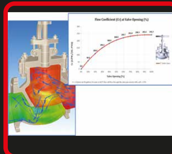
Equipment fluid dynamics characterisations (for CV curve) using 3D CFD
