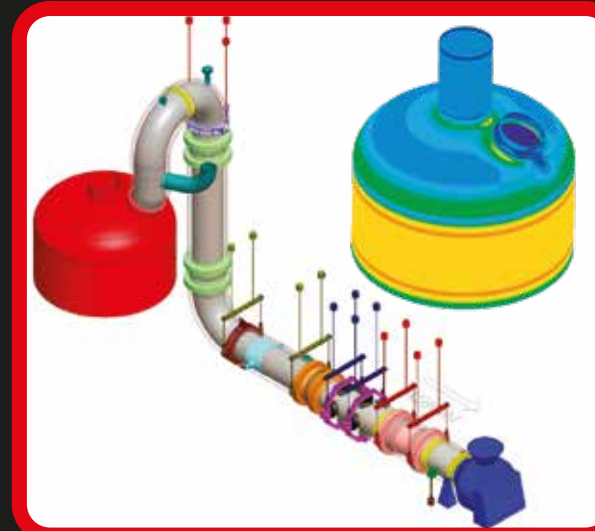
PRT Gas Turbine Recovery Train Design and Analysis
