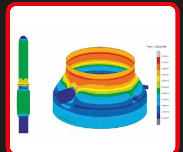
Significant damage assessment of Creeping cone penetration on major vessel
