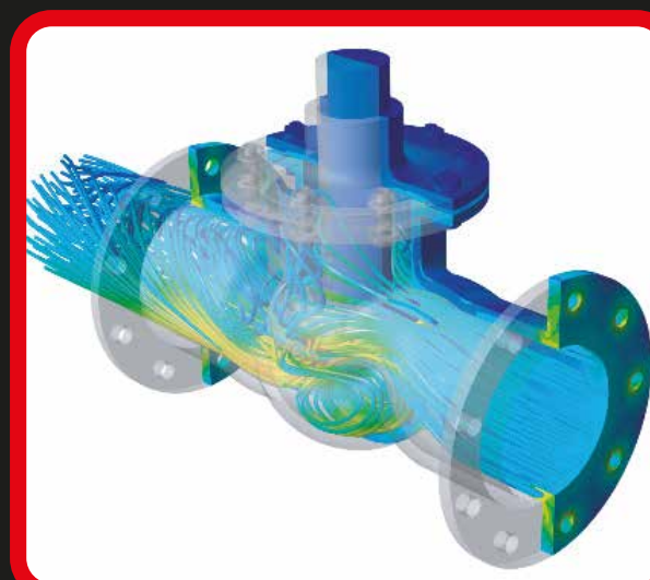
Fluid Structure Interaction (fluid and mechanical) of new valve design using FEA and CFD
